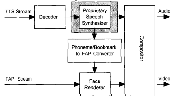
Figure 8: Block diagram showing the integration of a proprietary Text-to-Speech Synthesizer into an MPEG-4 face animation system.
