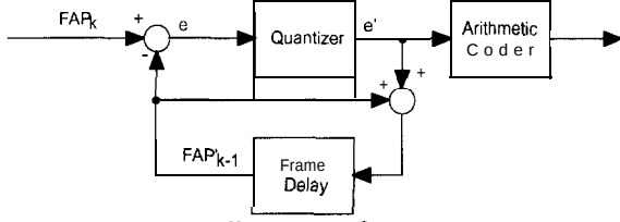
Figure 5: Block diagram of the encoder for FAPs.
