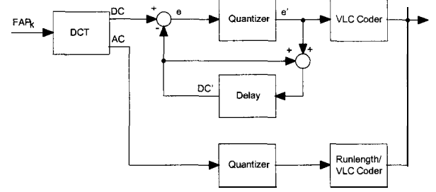
Figure 6: Block diagram of the FAP encoder using DCT. DC coefficients are predictively coded. AC coefficients are directly coded.
